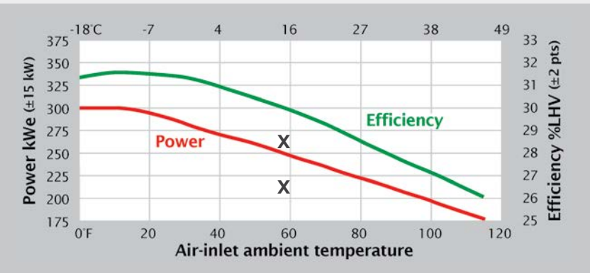
ELECTRICAL OUTPUT GRAPH SHOWS CHANGE IN POWER AND EFFICIENCY WITH TEMPERATURE
